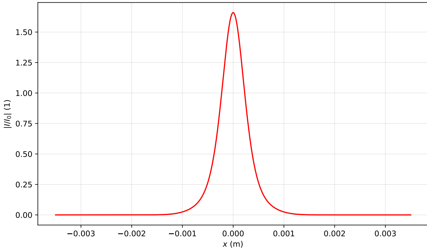
Intensity profile I(x, y = 0, z = 1.194)/I_0 , P_{in}=1.0P_{cr} , artificial time
